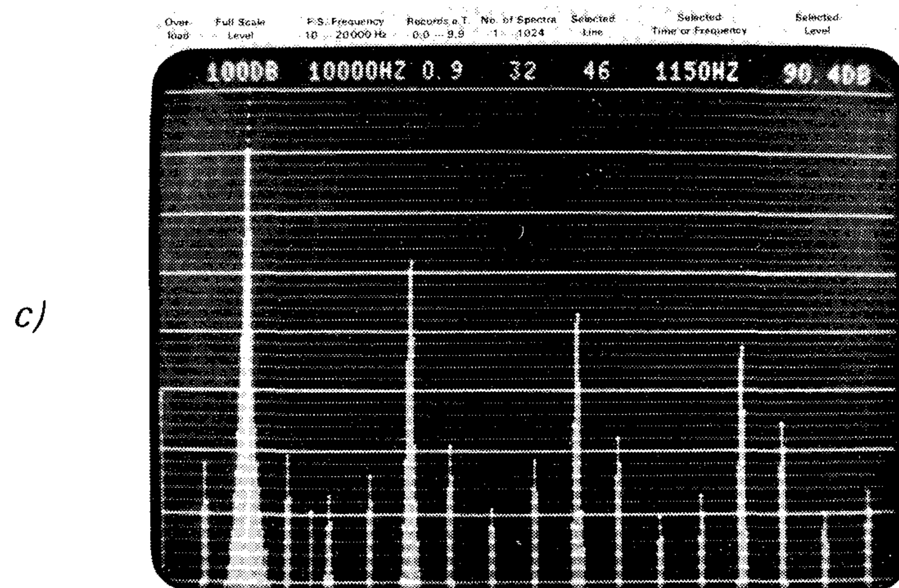
Fig.2. FFT analysis a) Triangular time signal RMS power spectrum b) with antialiasing filter c) without antialiasing filter
