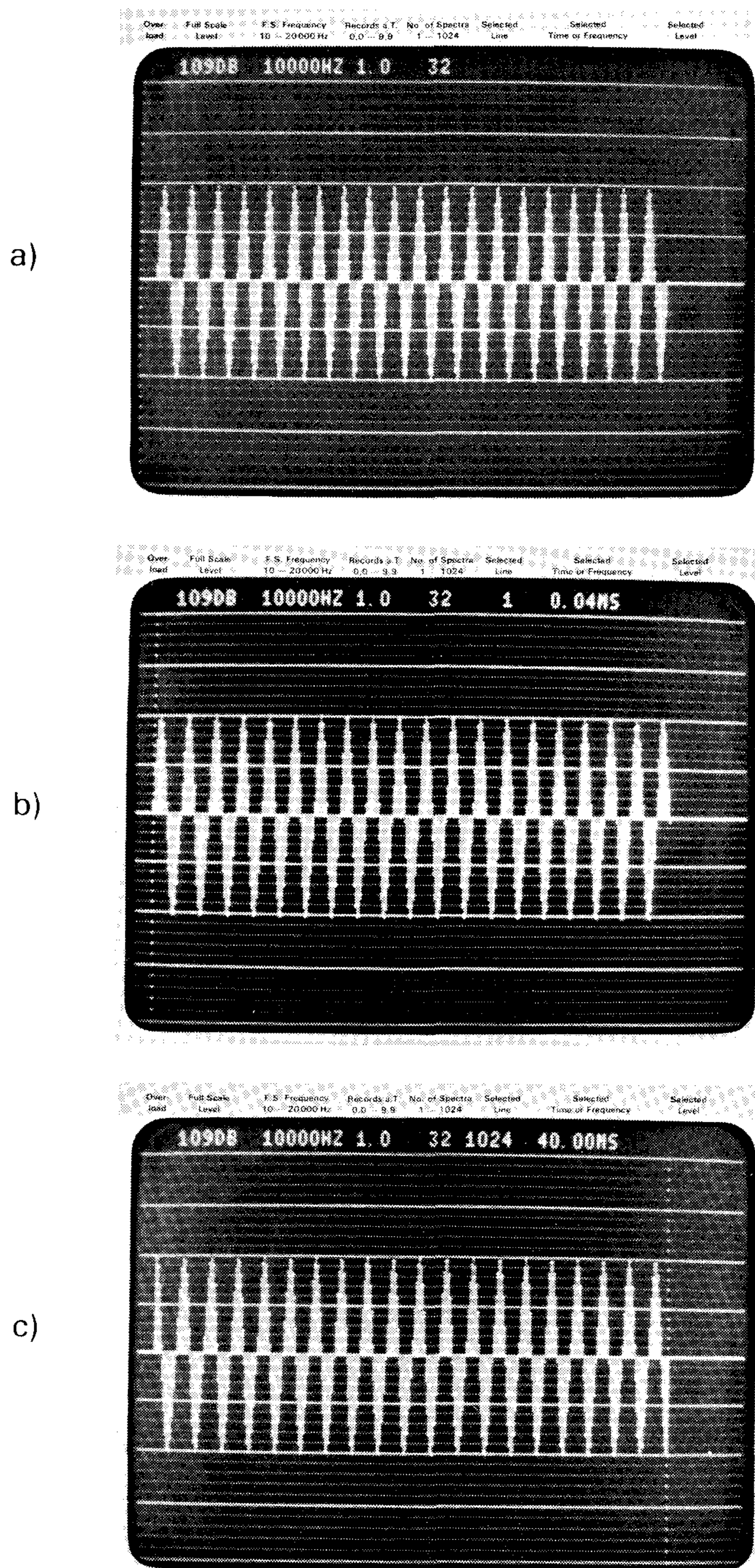
Fig.7. FFT analysis of sinusoidal time signals using different window functions. Number of periods in time memory: a) integer, b) and c) half-integer but different phases
