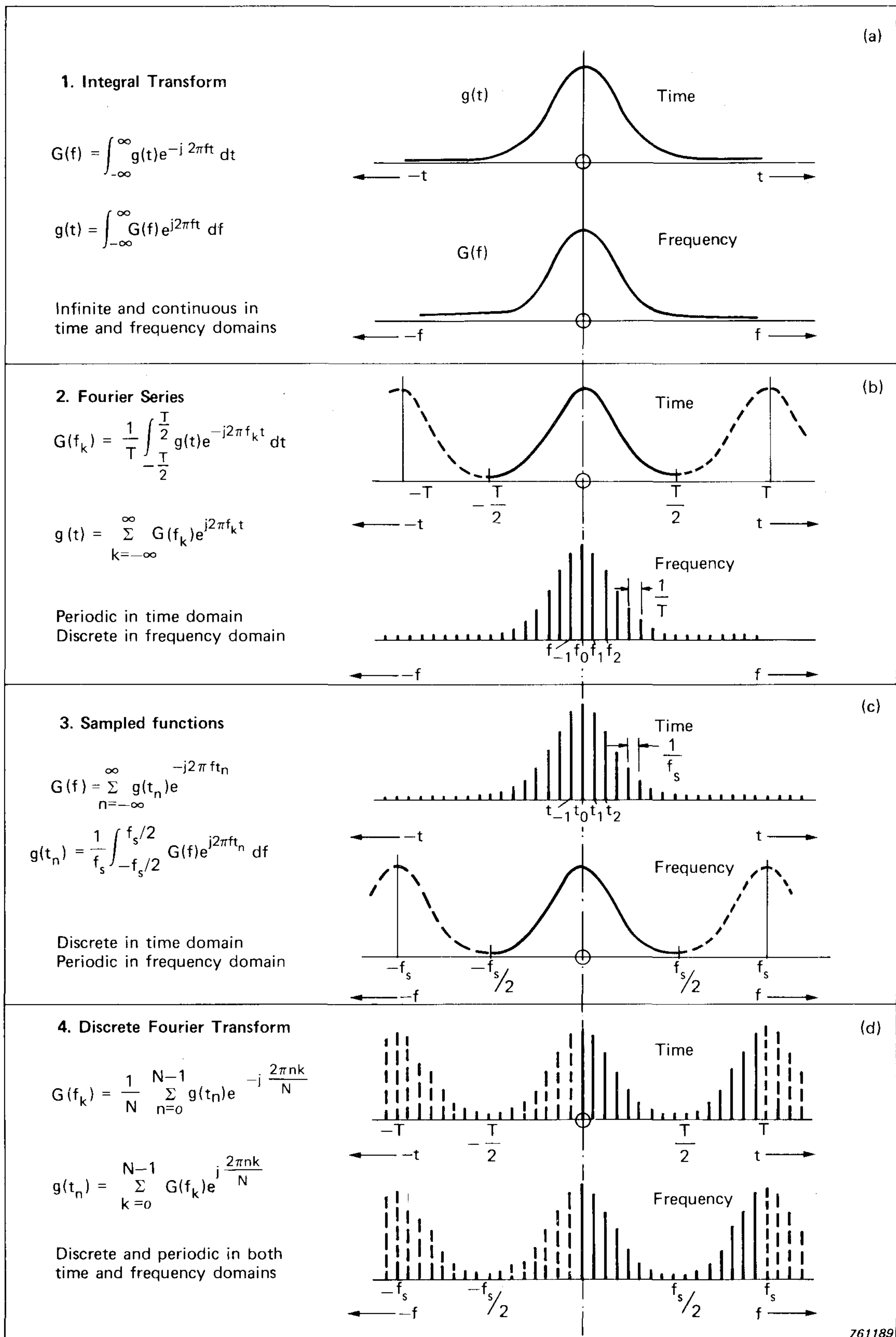
Fig. 1. Various forms of the Fourier Transform
