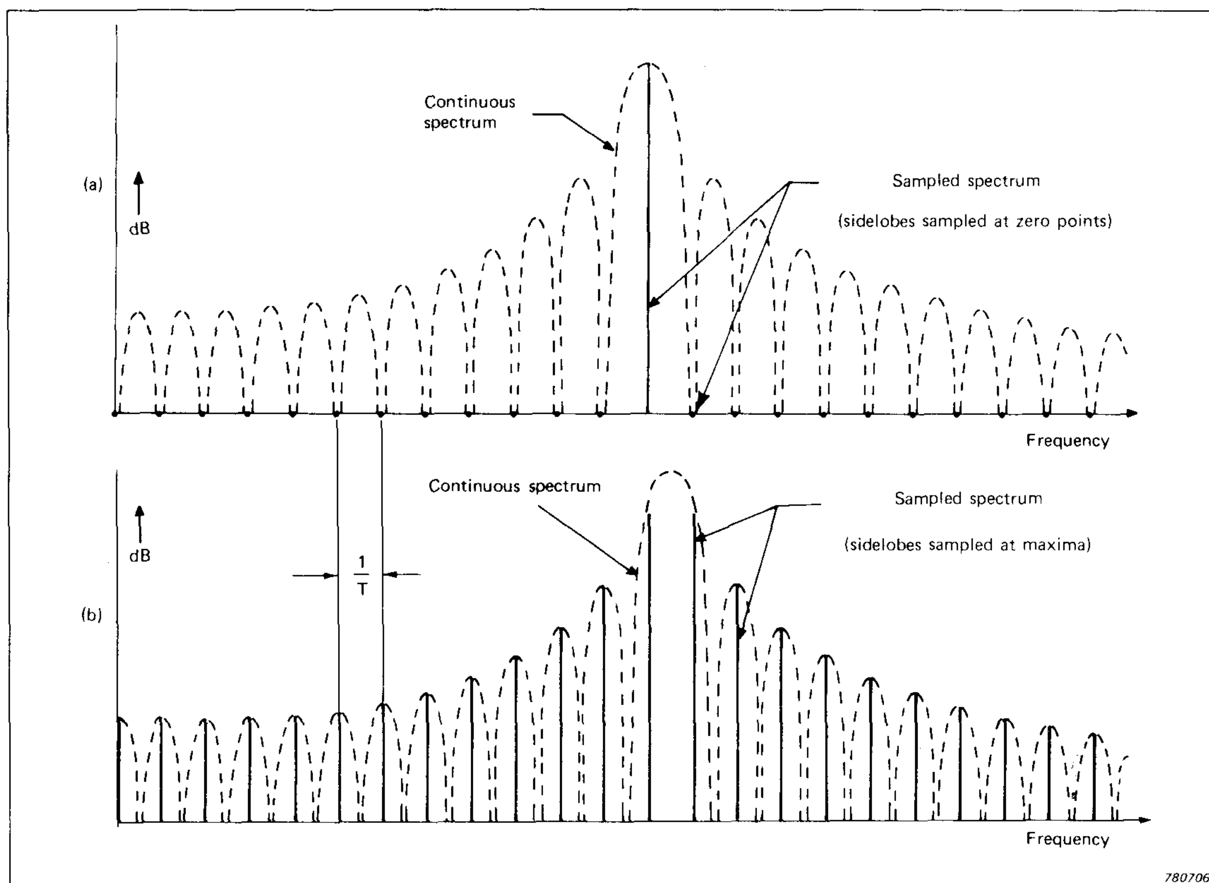
Fig.6. Frequency sampling of the continuous spectrum of a time limited sinusoid. Number of periods within the time window: a) integer, b) half-integer
